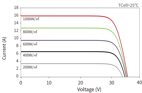
Current-Voltage Curves (48QL6-DV 475W)
