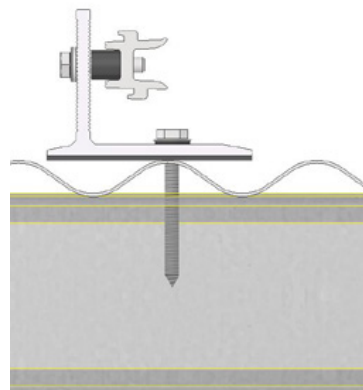
Fixing through corrugated roof sheet on purlin
