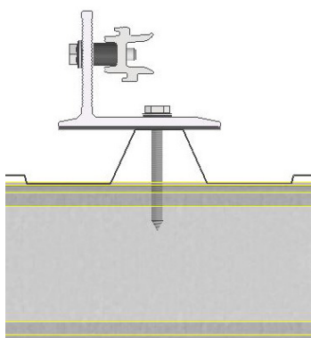
Fixing through trapezoidal roof sheet on purlin
