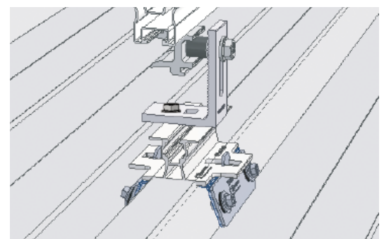
Portrait &amp; Landscape with SingleFix HU pre-assembled
