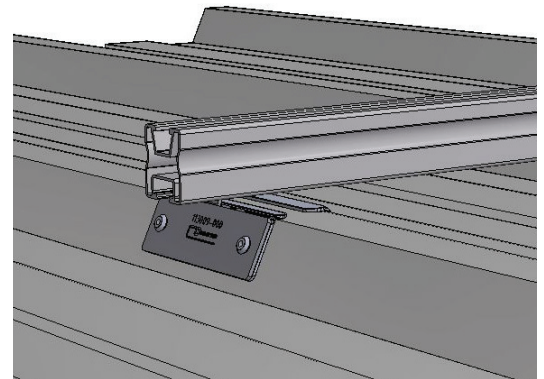
Portrait with SingleFix
