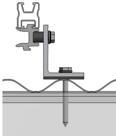
Fixing through corrugated roof sheet on purlin
