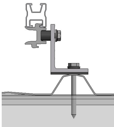
Fixing through trapezoidal roof sheet on purlin
