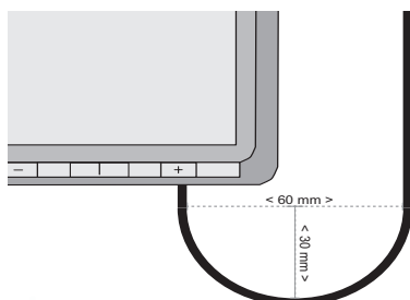
Fig. 6 Minimum Cable dDistance
