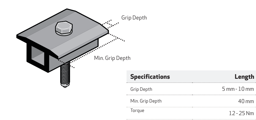
Fig. 1 Clamp Specifications
