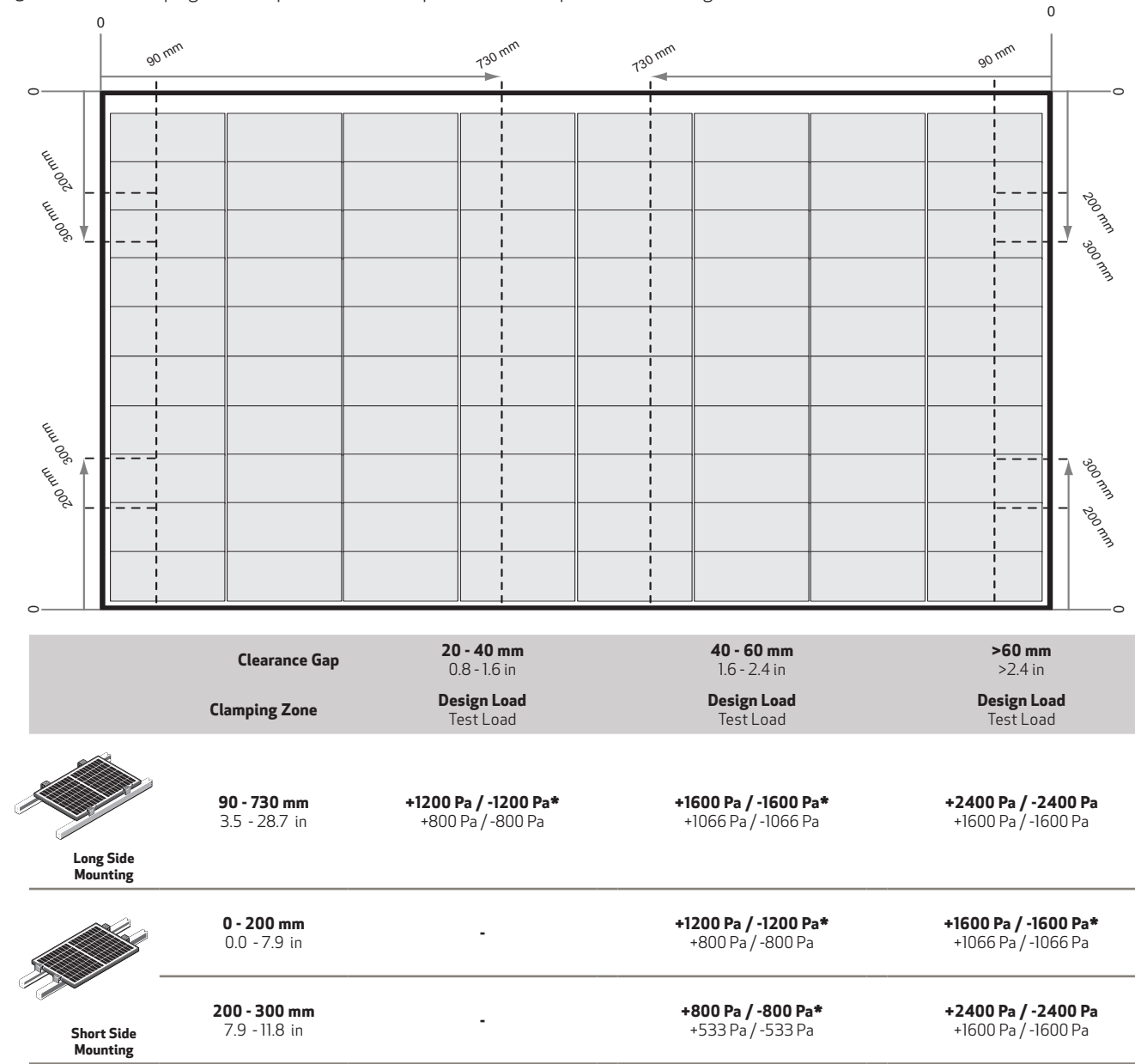
Fig. 4-2 Clamping of REC Alpha Pure-R Series panels with Rails parallel to the Long Side of the Panel
