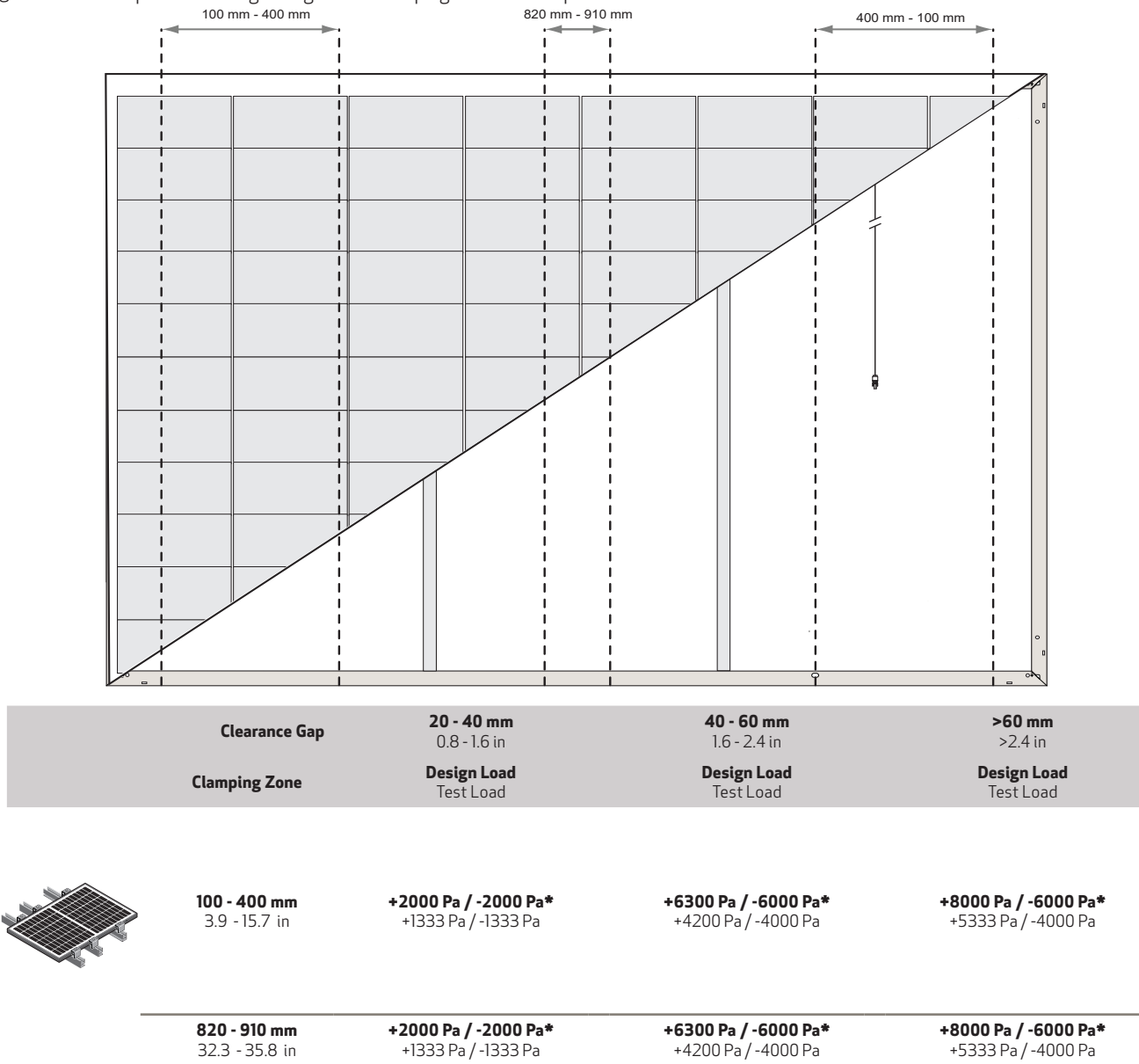
Fig. 5-4 Six-point mounting configuration clamping zones: REC Alpha Pure-RX Series
