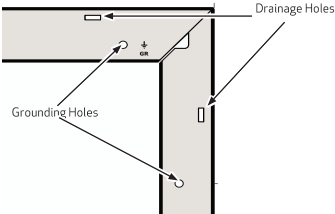
Fig. 5 Drainage and Grounding Holes
