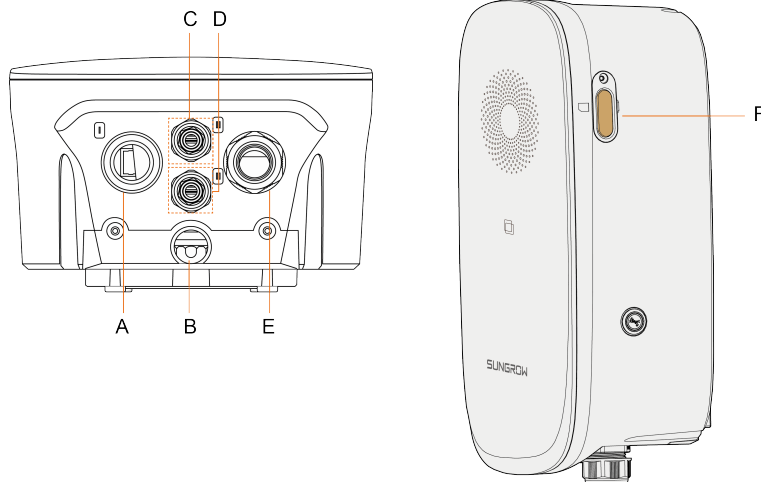
figure 1-2 Terminal Diagram
