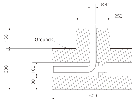
figure 2-5 Front view (unit: mm)
