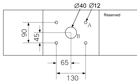
figure 2-6 Top view (unit: mm)
